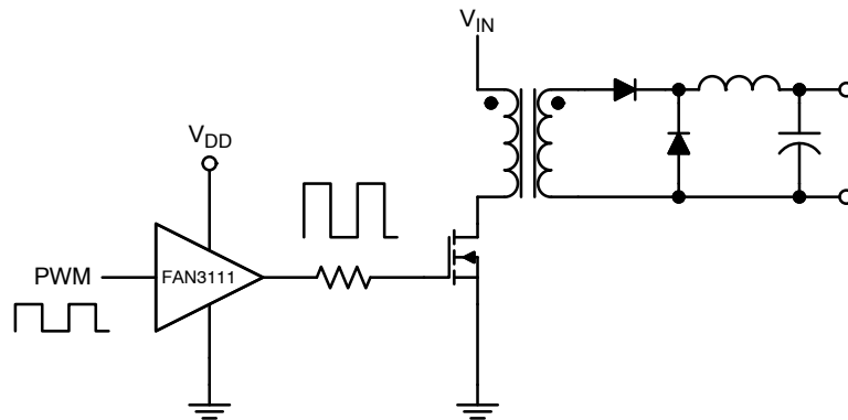
Figure 42. Driver for Forward Converter Low-Side Switch
